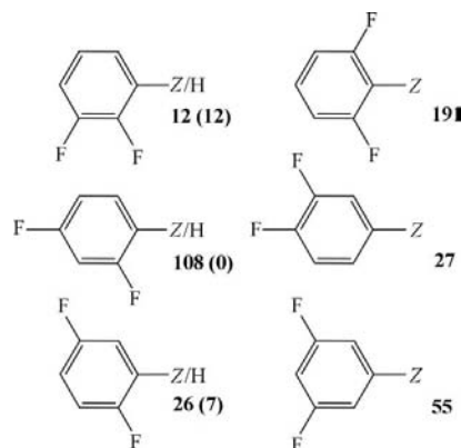
Figure 1 Relative abundance of difluorobenzene fragments in the CSD (Version 5.29, January 2008 updates). X = any element and Z = any element but H.
